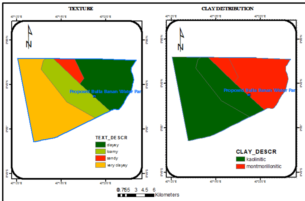
Figure 3.4: Soil map of the project area
